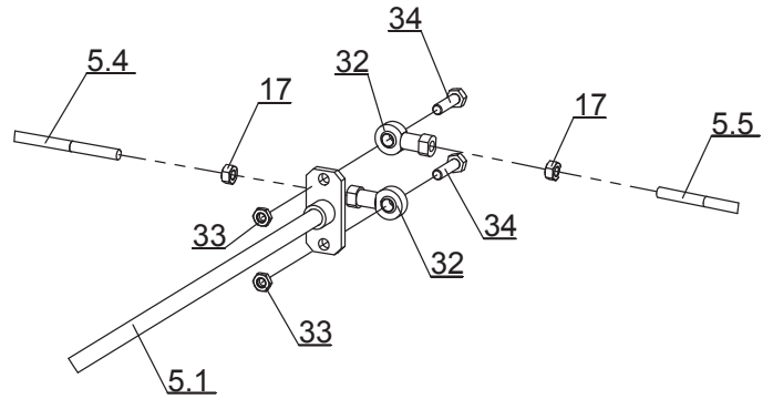
LOCAL VIEW B
